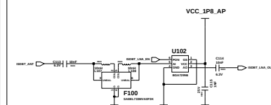
ISDBT_FRONTEND
