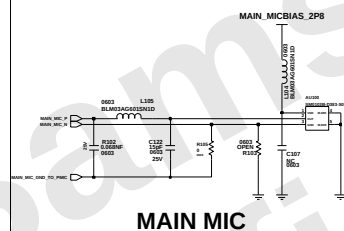
MAIN MIC
