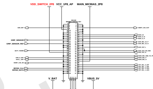
SUB PCB IF CONNECTOR
