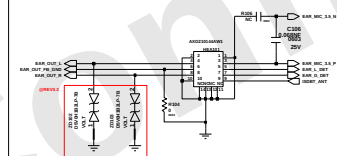
EARJACK CONNECTOR
